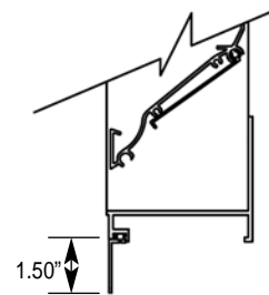
Flange Detail
