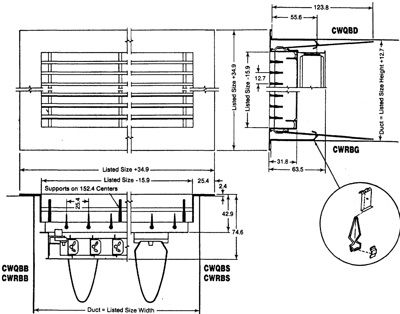
DIMENSIONS LISTED IN MILLIMETERS
