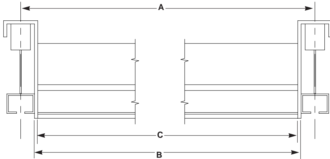
CHANNELAIRE SIDE VIEW
