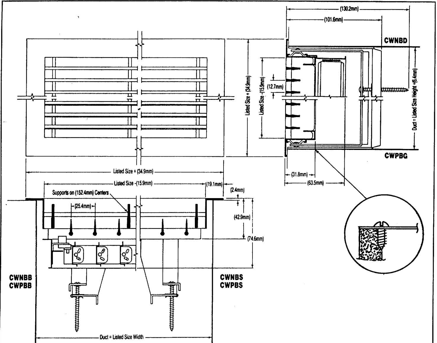
DIMENSIONS LISTED IN MILLIMETERS
