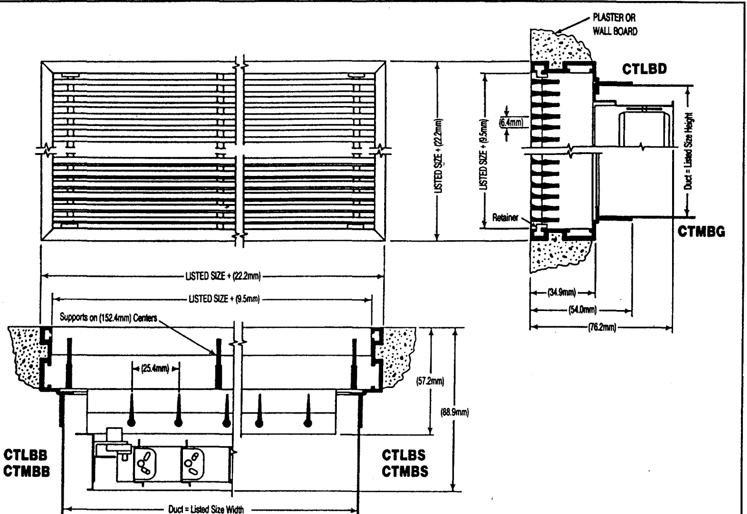
DIMENSIONS LISTED IN MILLIMETERS
